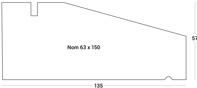
Hardwood Cill
